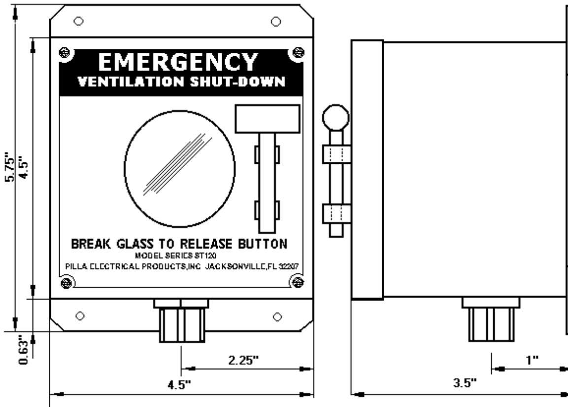
PILLA MODEL ST120SN4XS304SL VENTILATION SHUT-DOWN BREAK GLASS STATION
