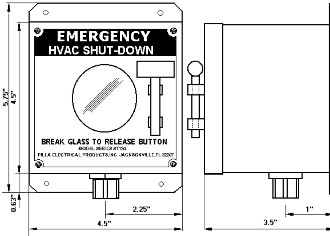
PILLA MODEL ST120SN4XS304SL HVAC SHUT-DOWN BREAK GLASS STATION
