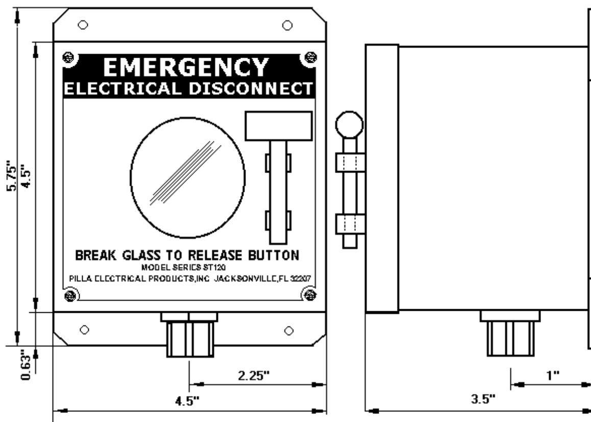
PILLA MODEL ST120SN4XS304 BREAK GLASS STATION
