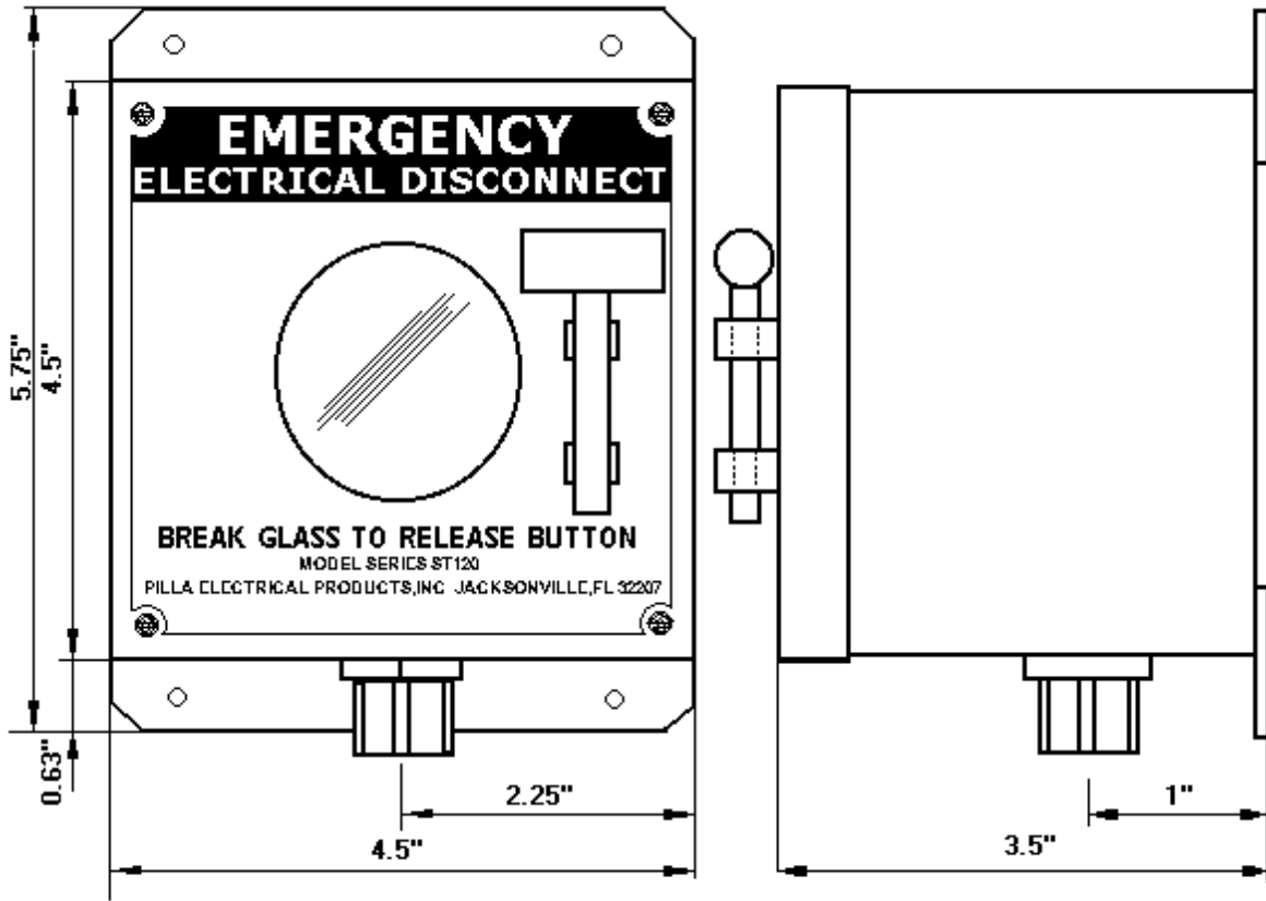
PILLA MODEL ST120SN4XA BREAK GLASS STATION
