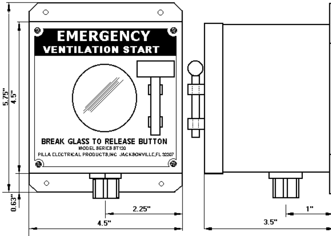
PILLA MODEL ST120SN4SL VENTILATION START BREAK GLASS STATION
