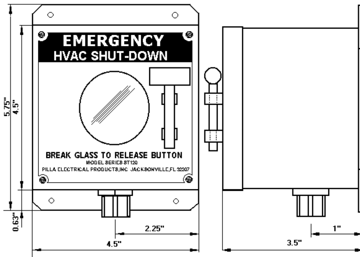
PILLA MODEL ST120SN4SL HVAC SHUT-DOWN BREAK GLASS STATION
