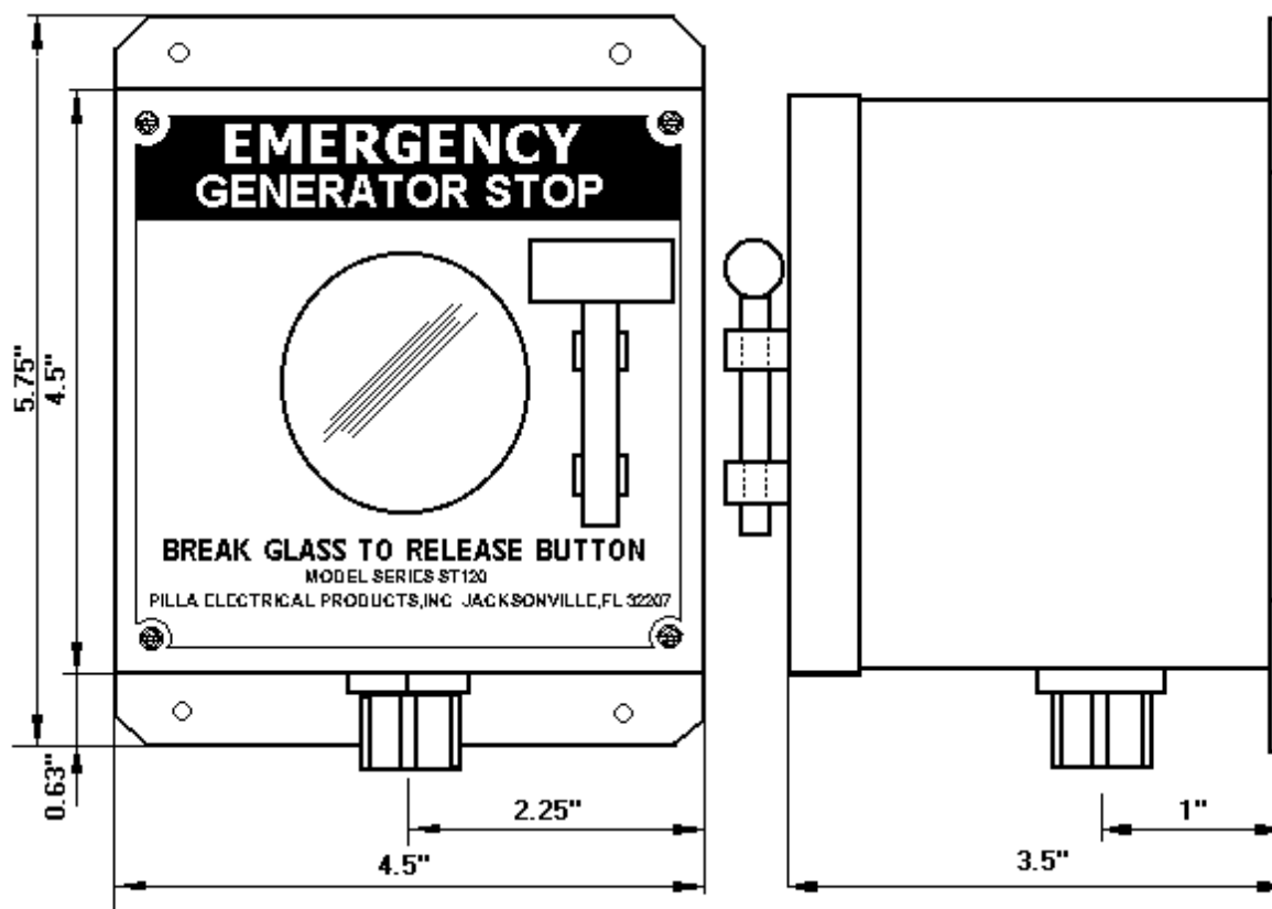
PILLA MODEL ST120SN4SL GENERATOR STOP BREAK GLASS STATION
