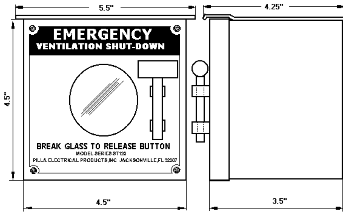
PILLA MODEL ST120SN3RSL (Ventilation Shut-Down) BREAK GLASS STATION
