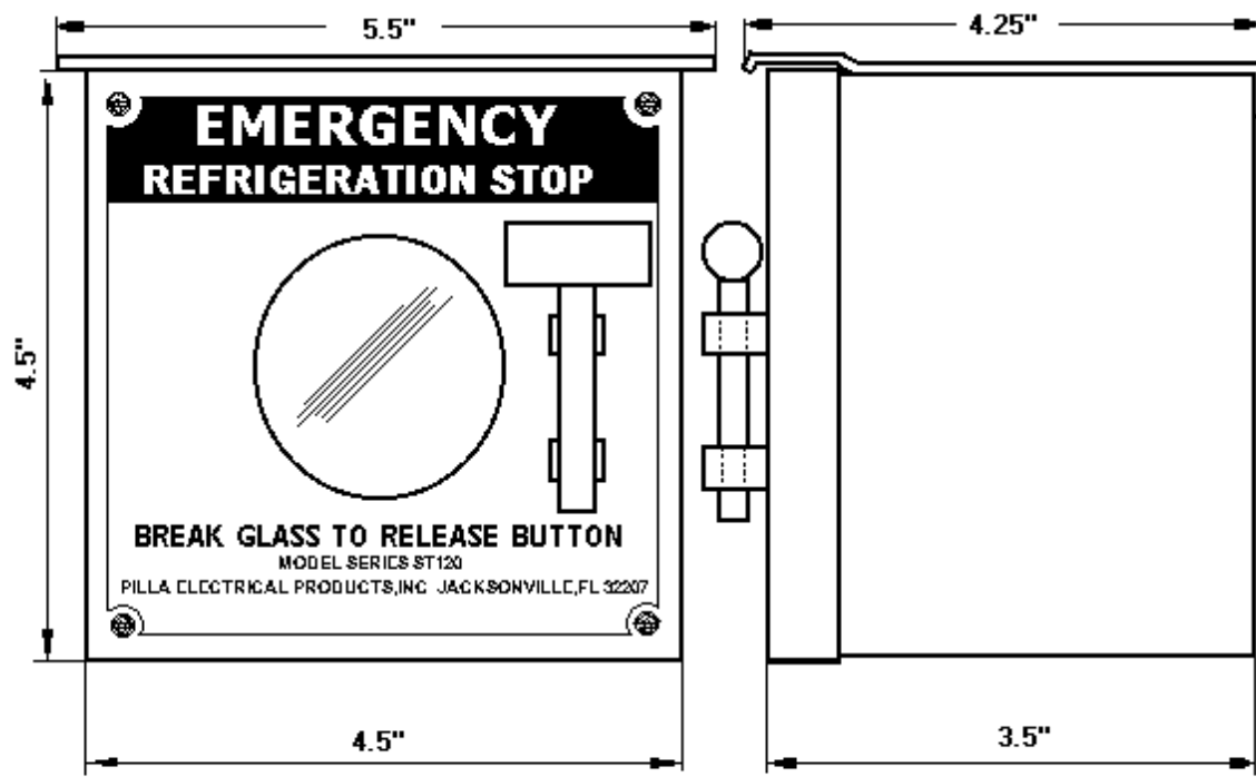
PILLA MODEL ST120SN3RSL (Refrigeration Stop) BREAK GLASS STATION
