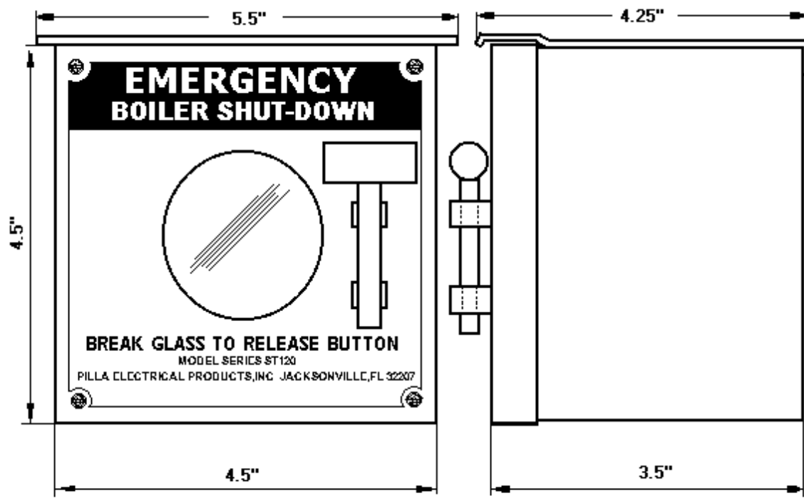
PILLA MODEL ST120SN3RSL (Boiler Shut-Down) BREAK GLASS STATION
