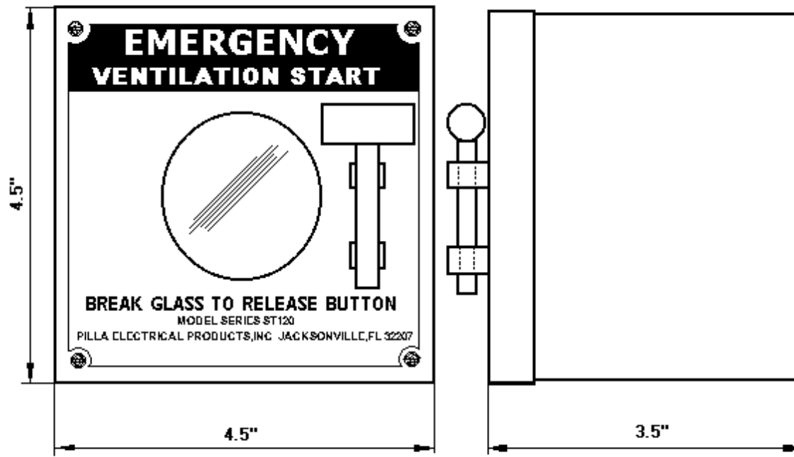
PILLA MODEL ST120SN1SL VENTILATION START BREAK GLASS STATION
