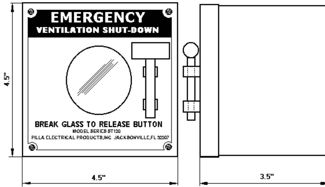
PILLA MODEL ST120SN1SL VENTILATION SHUT-DOWN BREAK GLASS STATION
