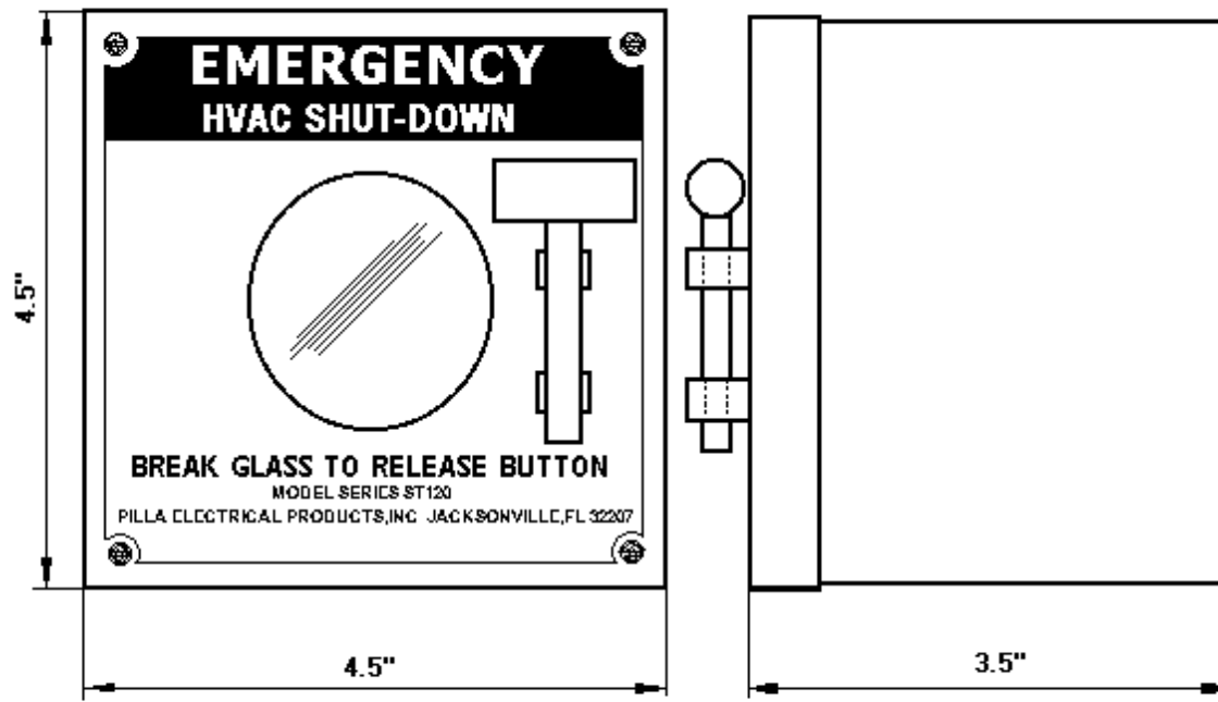
PILLA MODEL ST120SN1SL HVAC SHUT-DOWN BREAK GLASS STATION
