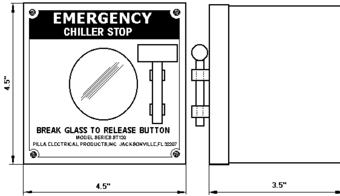
PILLA MODEL ST120SN1CHILLER STOP BREAK GLASS STATION
