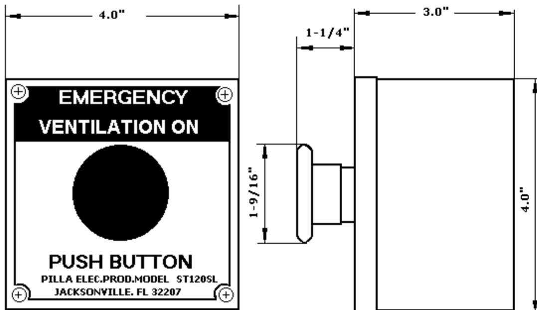
PILLA MODEL ST120SLN1 - VENTILATION ON PUSH BUTTON STATION
