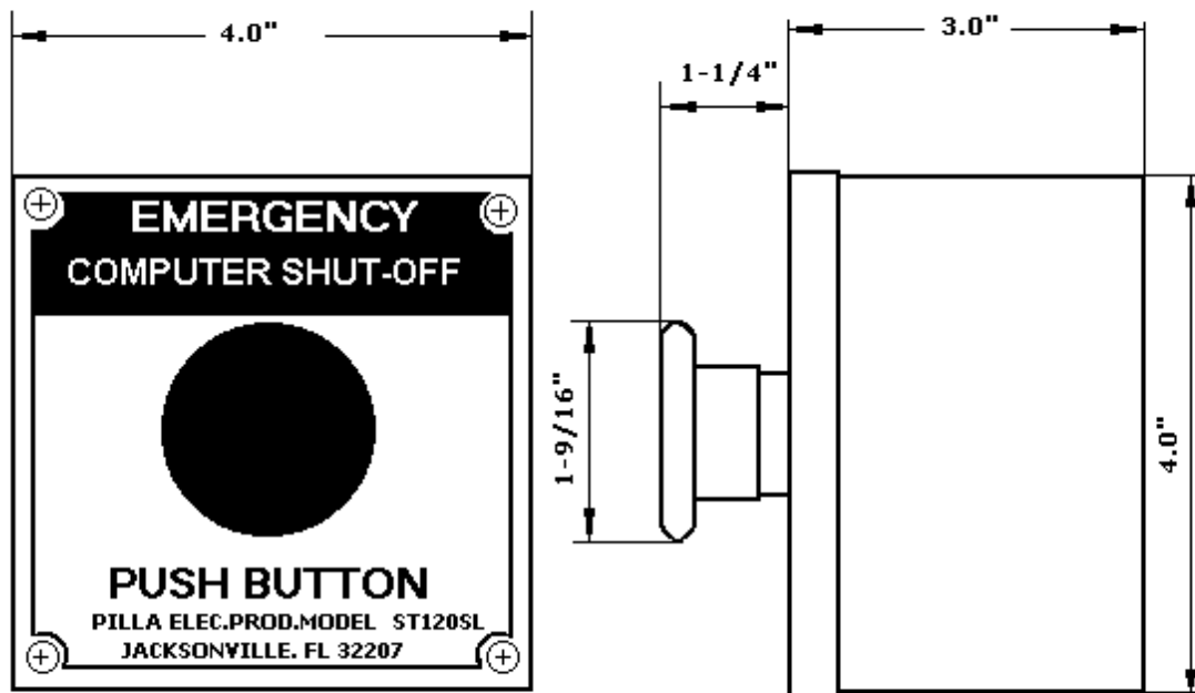
PILLA MODEL ST120SLN1-COMPUTER SHUT-OFF PUSH BUTTON STATION
