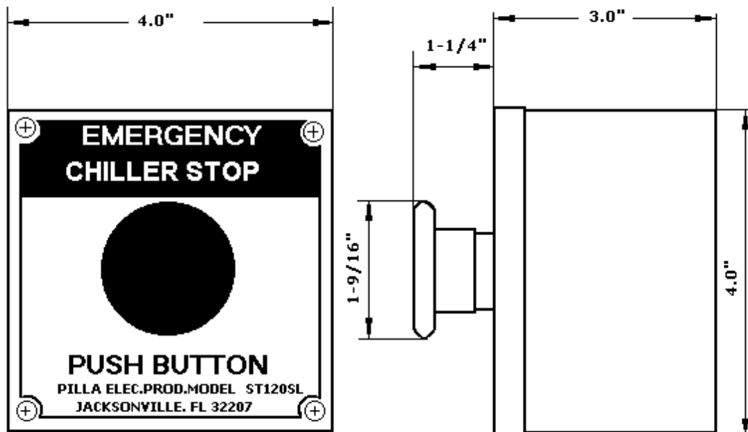
PILLA MODEL ST120SLN1-CHILLER STOP PUSH BUTTON STATION
