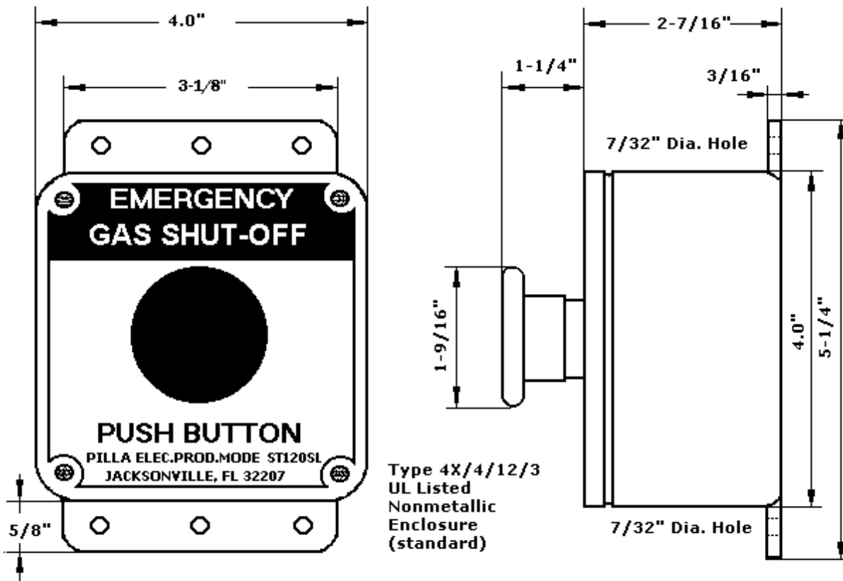
PILLA MODEL ST120SL - GAS SHUT-OFF PUSH BUTTON STATION
