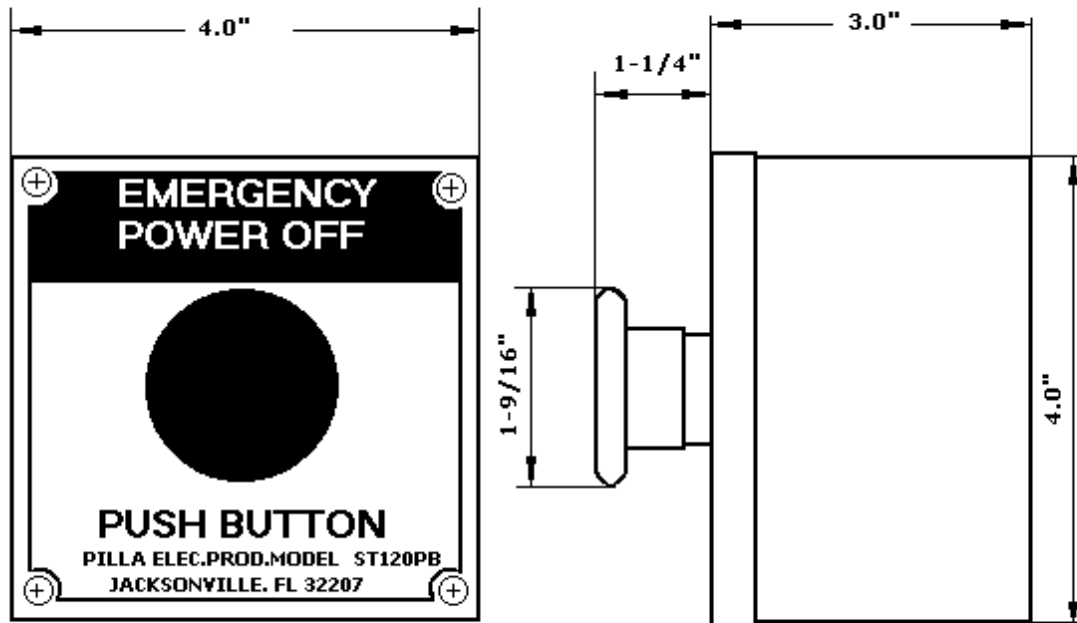
PILLA MODEL ST120PBN1 (Power Off) PUSH BUTTON STATION
