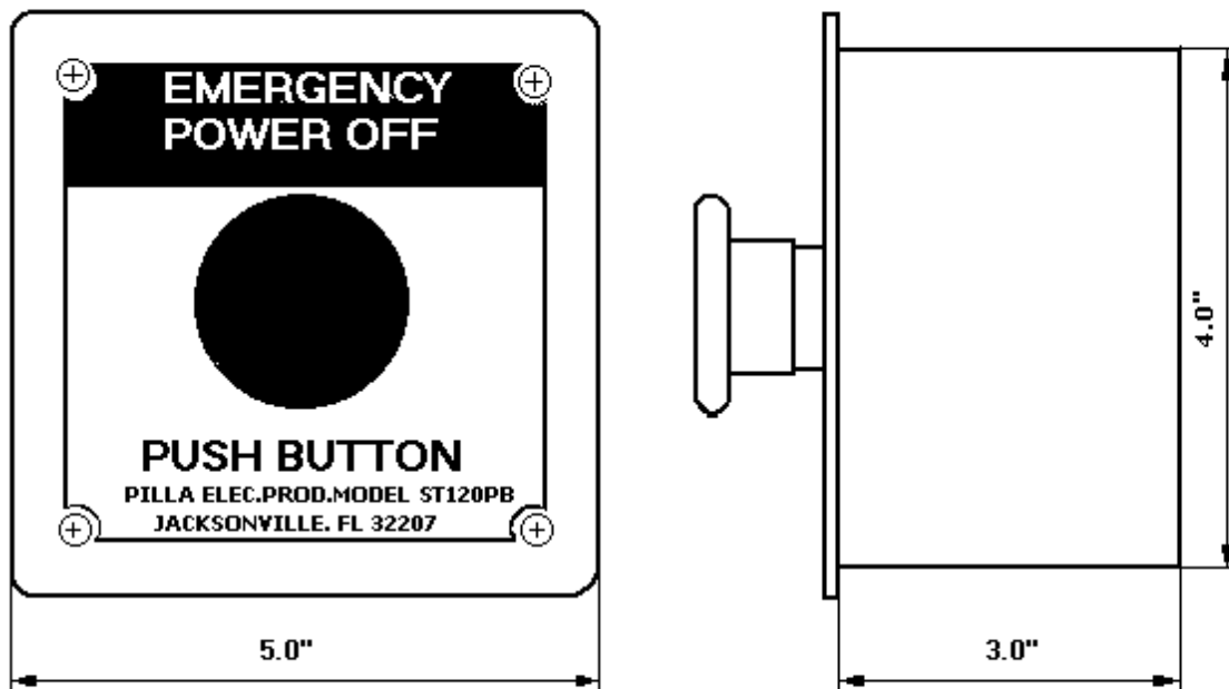
PILLA MODEL ST120PBF (Power Off) PUSH BUTTON STATION
