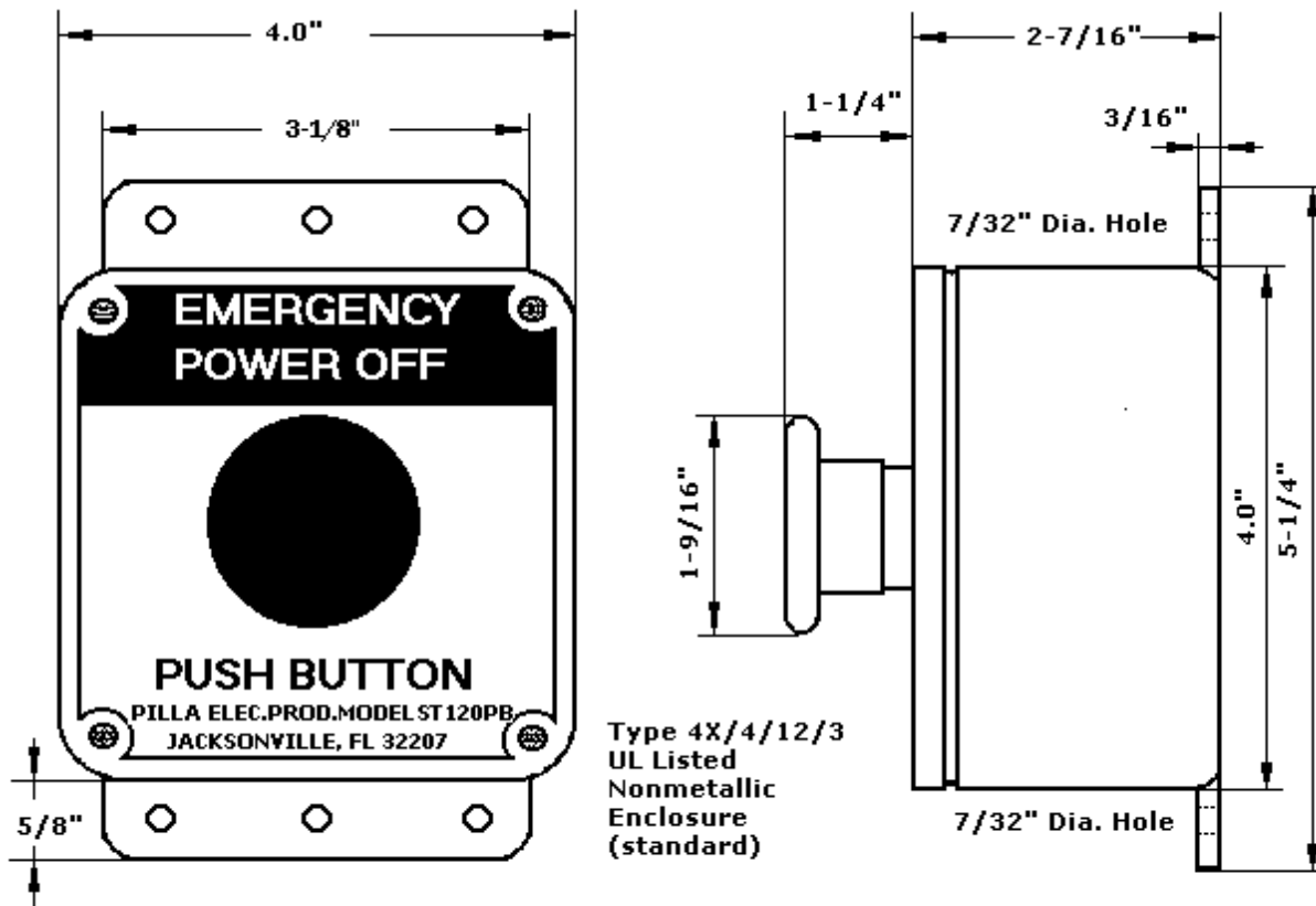
PILLA MODEL ST120PB (Power Off) PUSH BUTTON STATION
