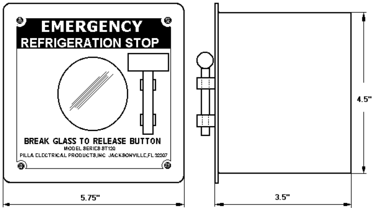
PILLA MODEL ST120FN4SL REFRIGERATION STOP BREAK GLASS STATION
