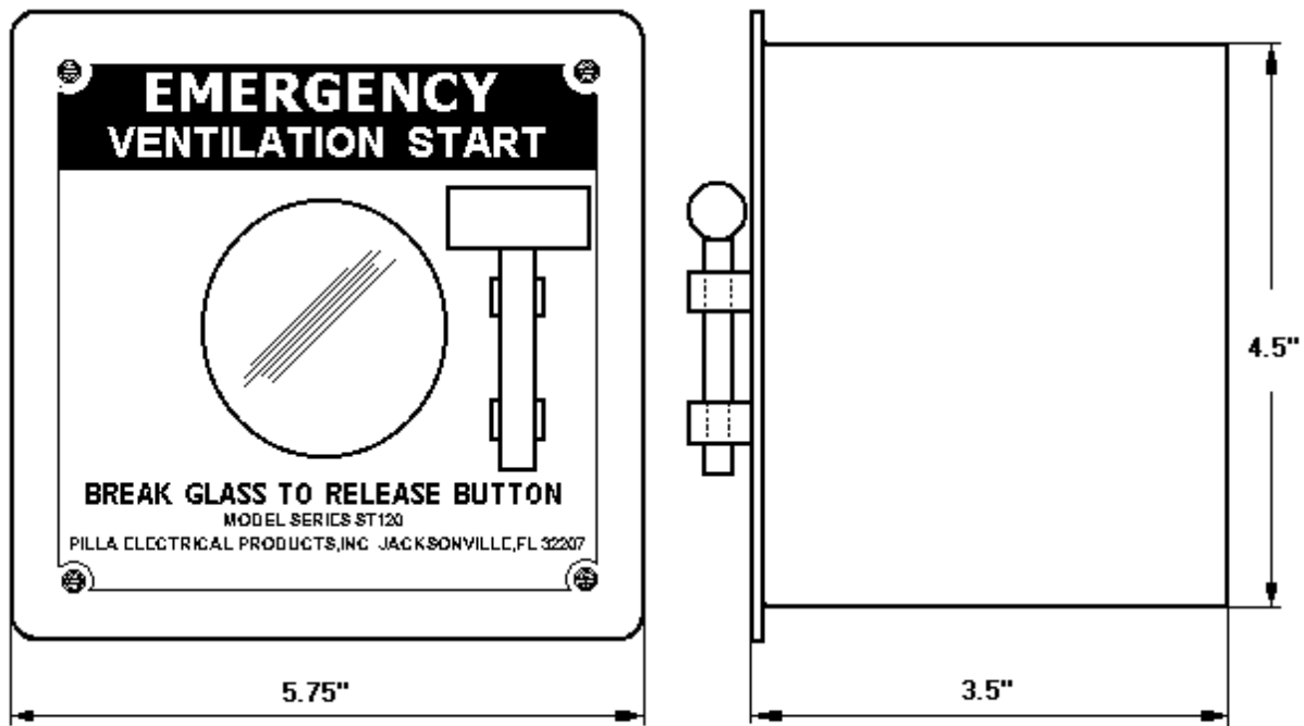
PILLA MODEL ST120FN1SL VENTILATION START BREAK GLASS STATION
