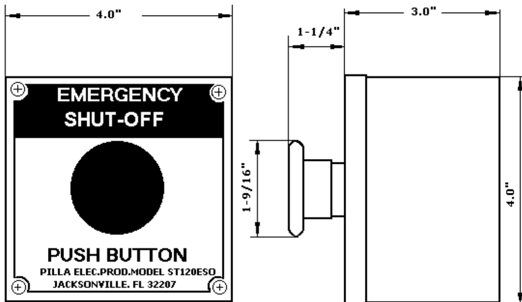
PILLA MODEL ST120ES0N1 (Emergency Shut-Off) PUSH BUTTON STATION
