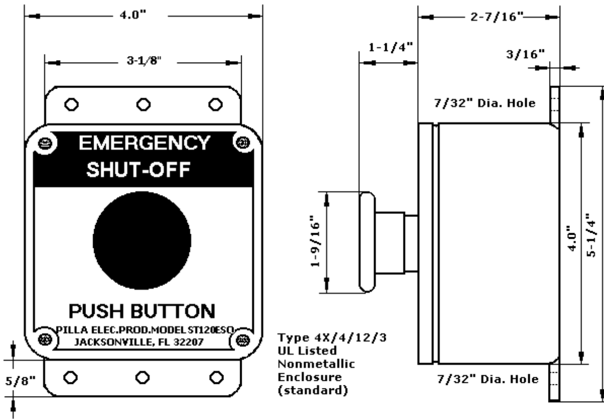
PILLA MODEL ST120ESO (Emergency Shut-Off) PUSH BUTTON STATION
