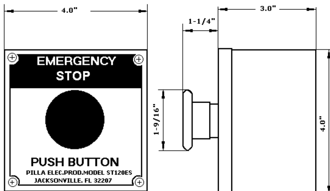
PILLA MODEL ST120ESN1 (Emergency Stop) PUSH BUTTON STATION
