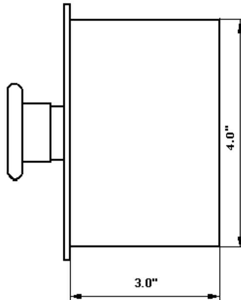
PILLA MODEL ST120ESFN1 (Emergency Stop) PUSH BUTTON STATION
