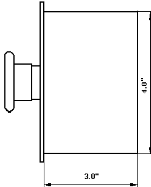
PILLA MODEL ST120ESF (Emergency Stop) PUSH BUTTON STATION
