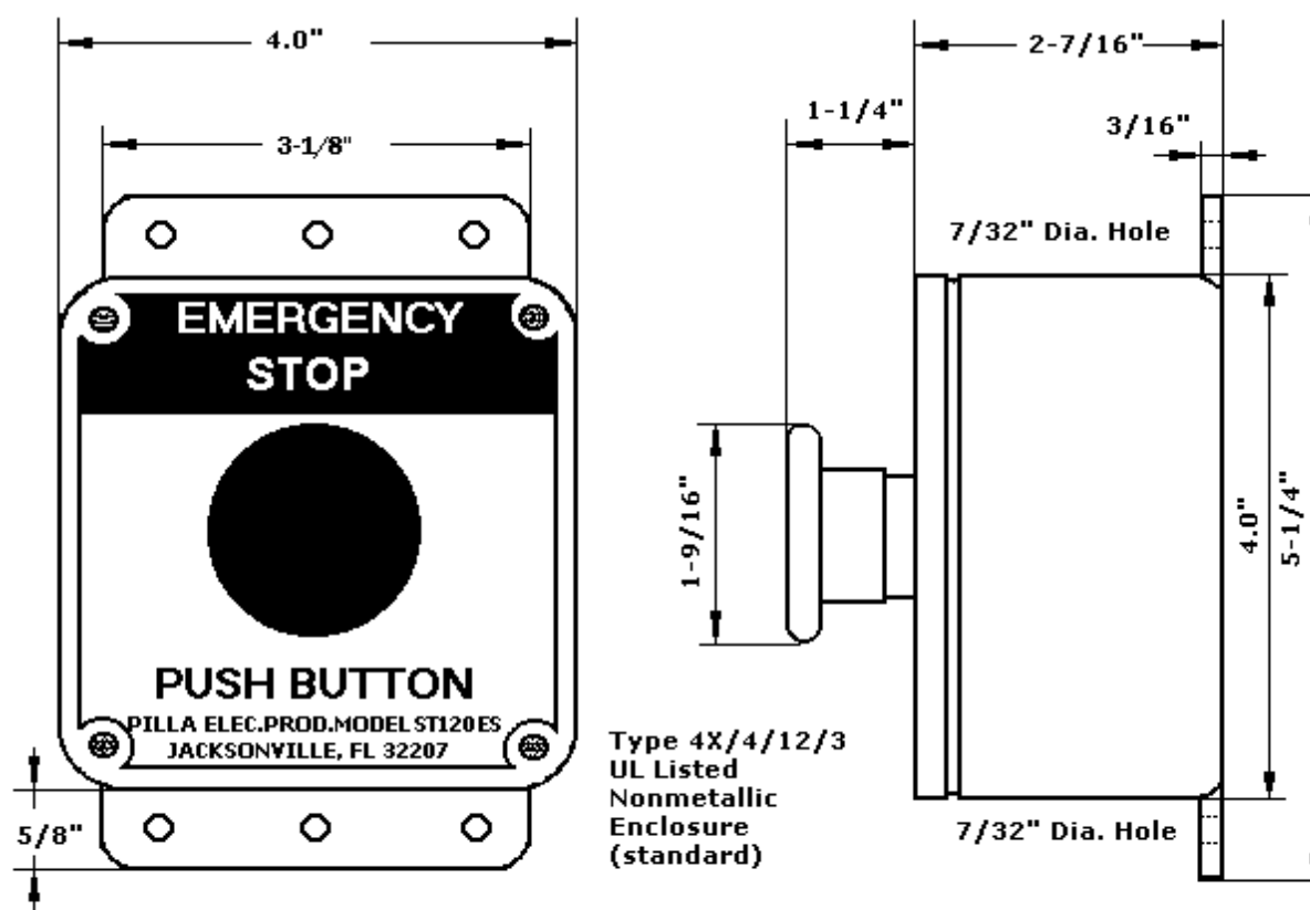
PILLA MODEL ST120ES (Emergency Stop) PUSH BUTTON STATION
