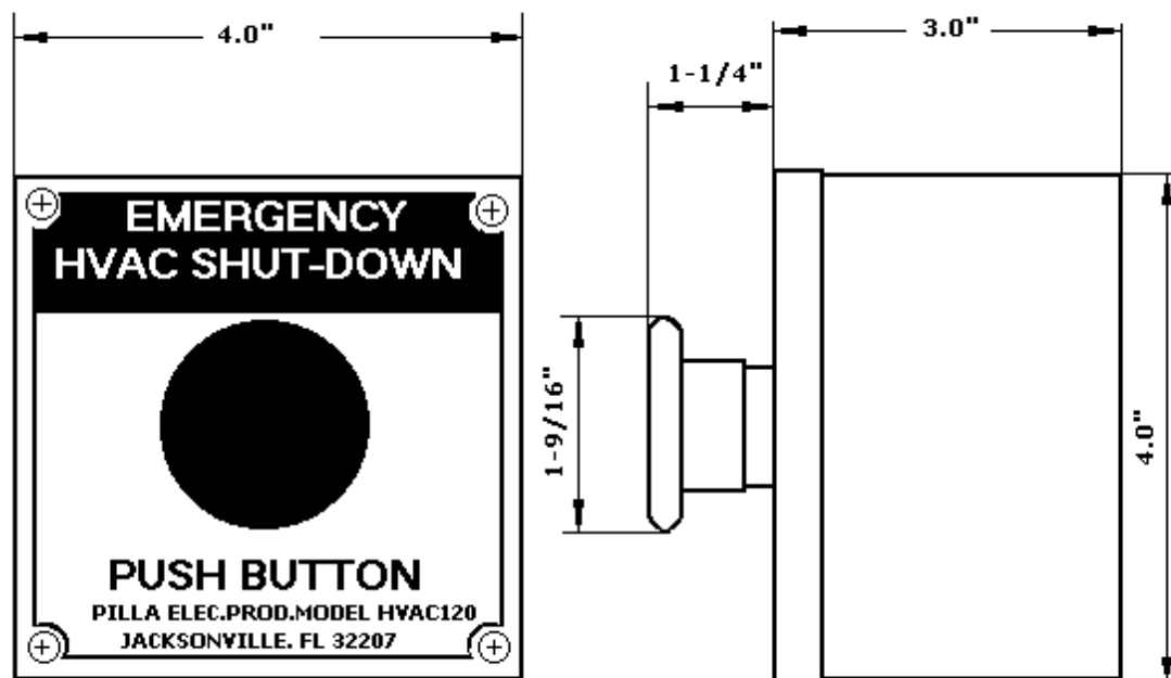
PILLA MODEL HVAC120N1 (Hvac Shut-Down) PUSH BUTTON STATION
