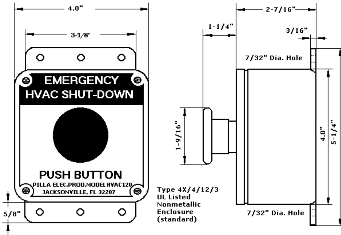
PILLA MODEL HVAC120 (Hvac Shut-Down) PUSH BUTTON STATION
