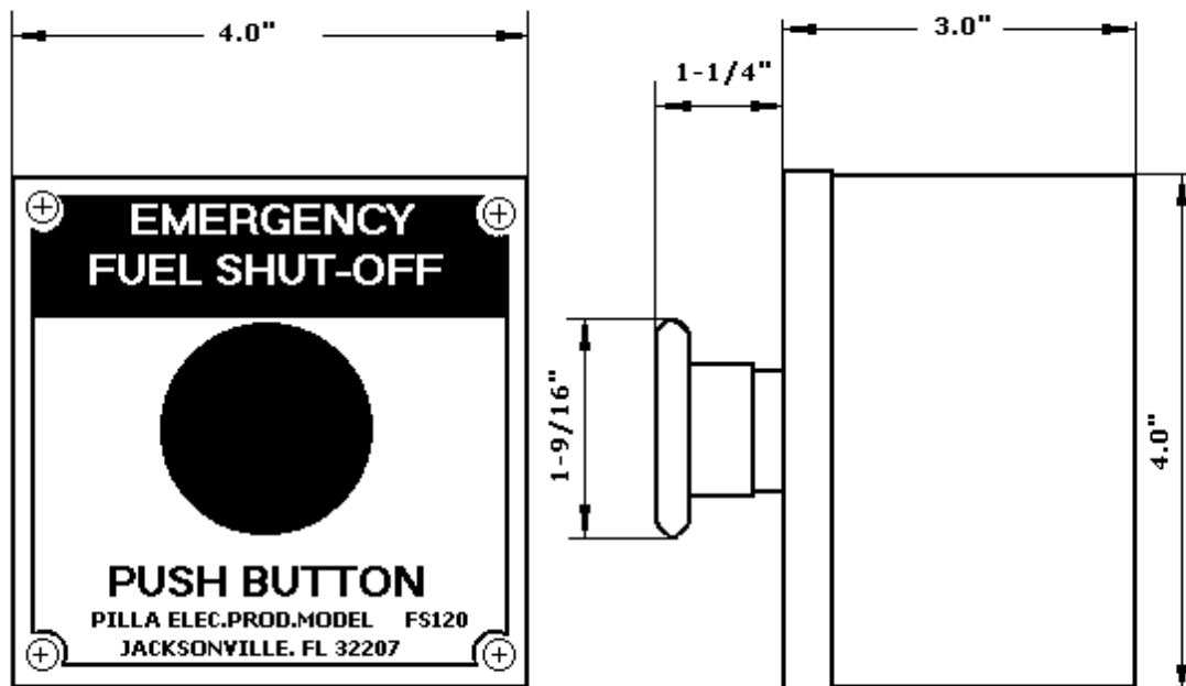
PILLA MODEL FS120N1 (Fuel Shut-Off) PUSH BUTTON STATION
