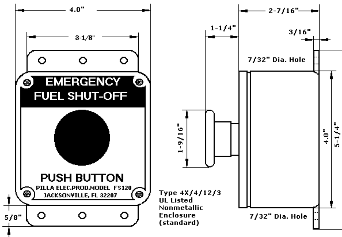
PILLA MODEL FS120 (Fuel Shut-Off) PUSH BUTTON STATION
