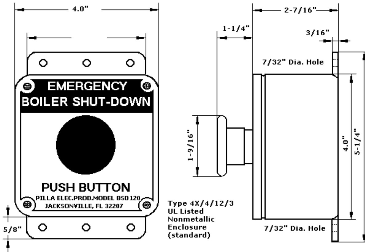
PILLA MODEL BSD120 (Boiler shut-down) PUSH BUTTON STATION
